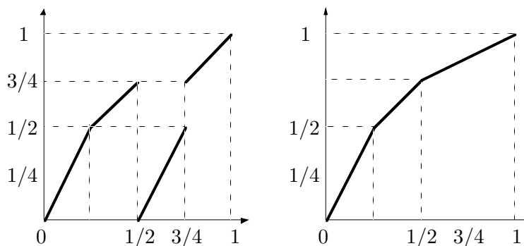
Figure 4.2. Left self-distributivity vs. associativity: action at \phi on the reals
