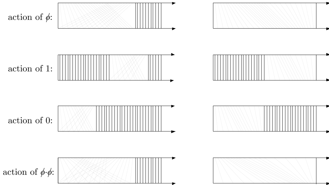
Figure 4.3. Left self-distributivity vs. associativity: rectangle diagrams
