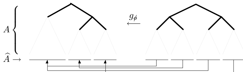
Figure 4.1. Action of G_{LD}^+ on the Cantor set
