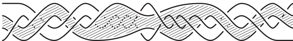
FIGURE 7. A ribbon in the counter-example of Figure 2
