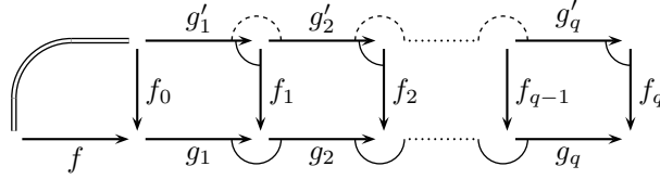
FIGURE 3. Proof of Lemma 3.4: starting from f in \mathcal{S}^\# and an \mathcal{S} -normal decomposition of g , we inductively build an \mathcal{S} -normal decomposition of fg .
