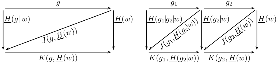
FIGURE 6. Proof of Lemma 5.1: attention! as long as the ambient category is not proved to be left-cancellative, the above diagrams should be taken with care.
