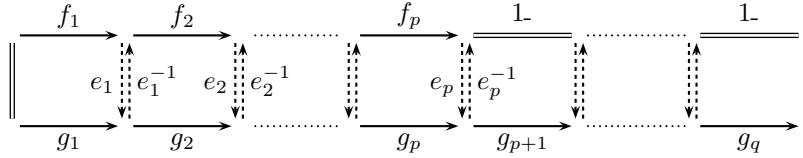
FIGURE 2. Deformation by invertible elements: invertible elements connect the corresponding entries; if one path is shorter (here we are in the case p < q ), it is extended by identity-elements.
