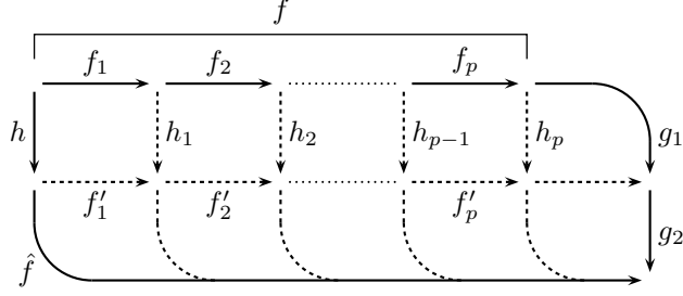
FIGURE 1. Proof of Lemma 2.6: whenever \mathcal{S}^\sharp generates the ambient category and is closed under right-complement, each relation h \preceq f g_1 g_2 leads to a relation of the form h_p \preceq g_1 g_2 and, therefore, the restricted form of greediness implies the general form.
